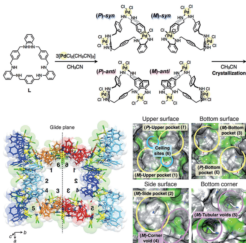
Figure 2. Top: Schematic representation of the formation of MMF (1) through cocrystallization of four stereoisomers of [\text{Pd}_3\text{LC}_6] , (P)-syn, (M)-syn, (P)-anti, and (M)-anti forms. Bottom: Each individual binding pocket, void, and site is numbered on the solvent-excluded molecular surfaces of the pore.
