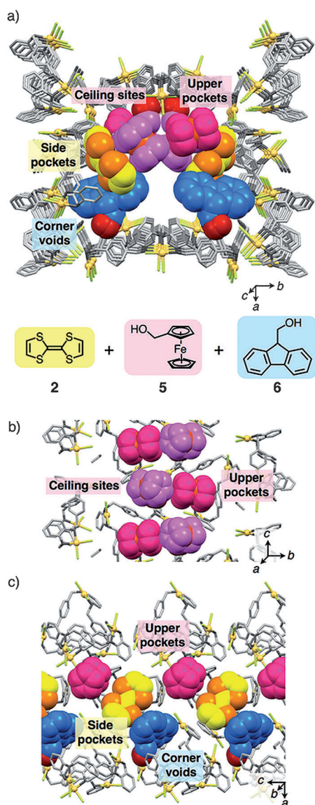
Figure 5. Crystal structure [19] of a ternary system composed of 2 (side pockets with 56 % occupancy), 5 (upper pockets and ceiling sites with 63 % and 60 % occupancies, respectively), and 6 (corner voids with 51 % occupancy) in MMF ( 1 ) (MMF: stick model, each guest: CPK model). a) The pore structure and b) the upper and c) the side surface structures of the ternary system.
